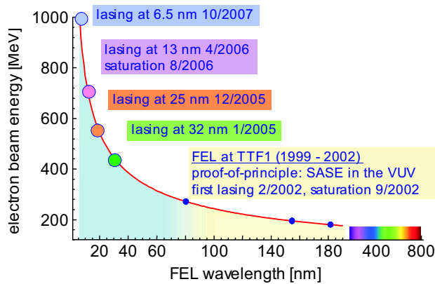
Figure 6: Evolution of the FLASH beam energy and the SASE wavelength.
