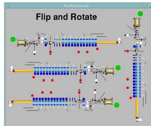
Figure 2: Flip and rotate options. The items shown were designed with the MEDM drawing tools.
