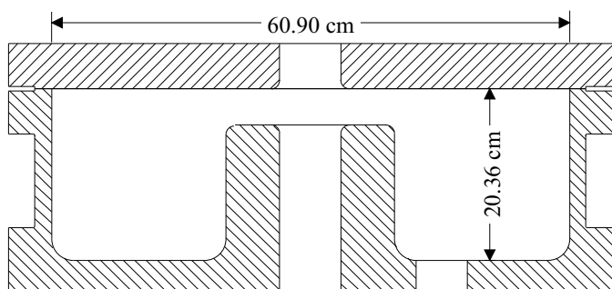
Fig. 1. 202 MHz Cavity Outline
