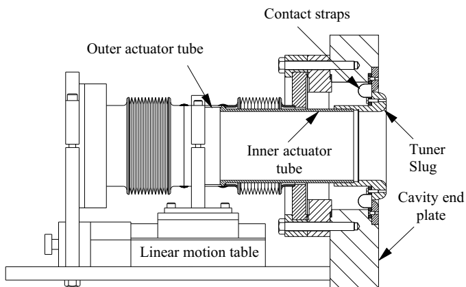
Fig. 2. Tuner Assembly
