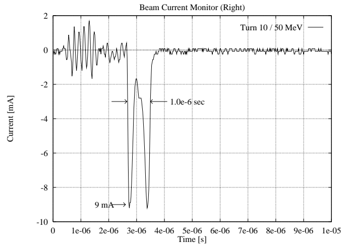
Figure 4. Electron beam pulse at the microtron exit.
