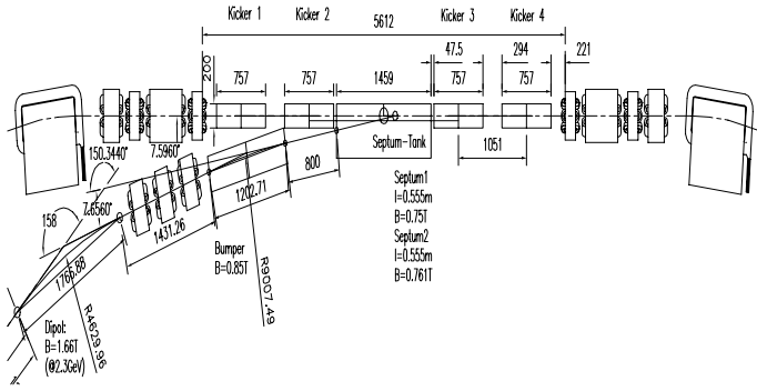
Figure 1. Storage ring injection region.
