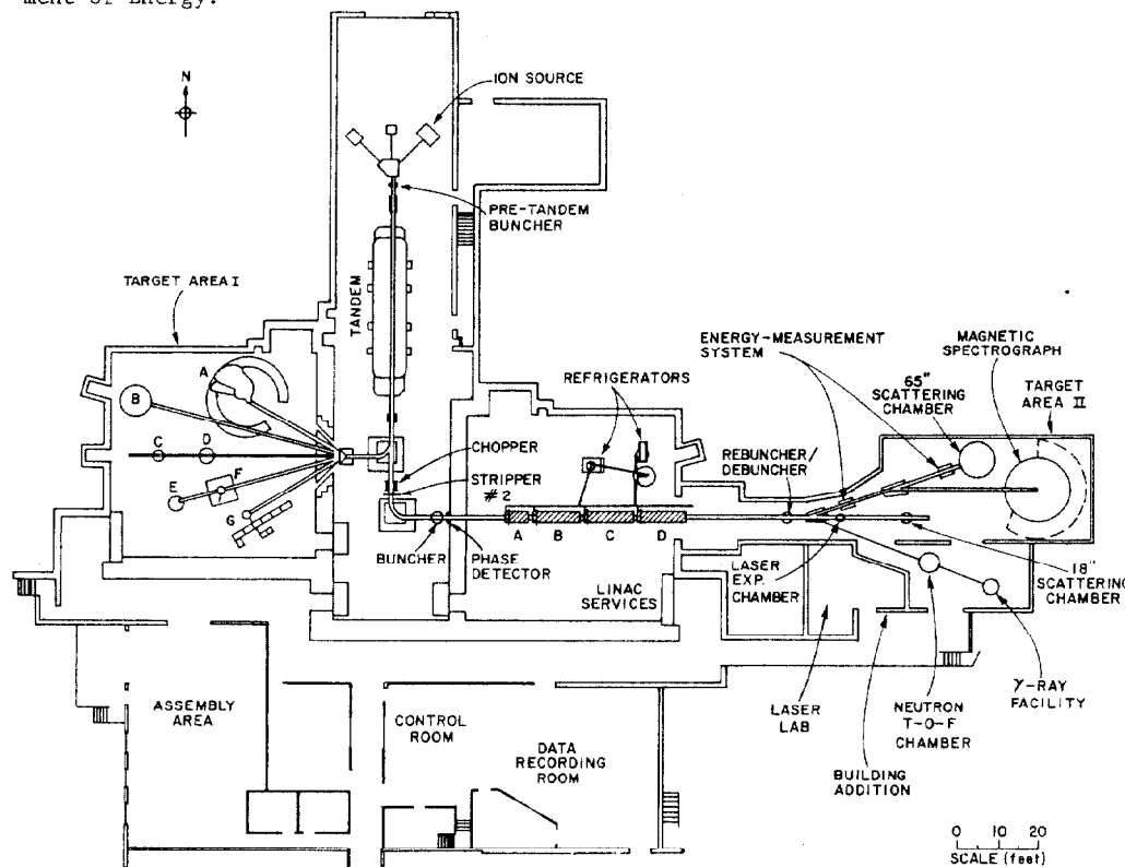
Fig. 1. Layout of the tandem-linac system at Argonne.
