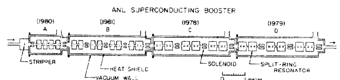
Fig. 2. Schematic of the superconducting linac.
