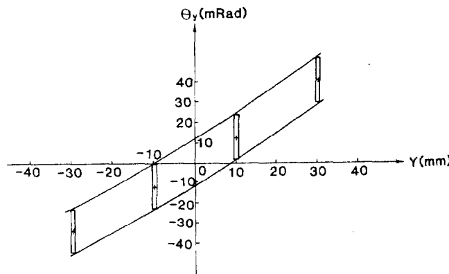
6. b. Phase space plot
