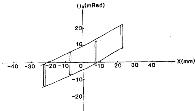
5. b. Phase space plot
