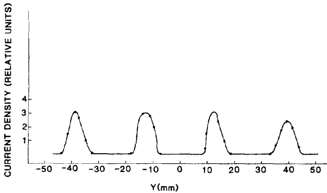
6. a. Charge collector emittance pattern
