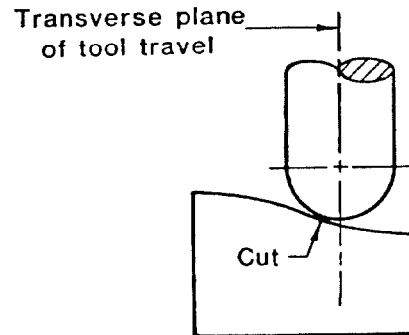
Fig. 5. Tool path error.
