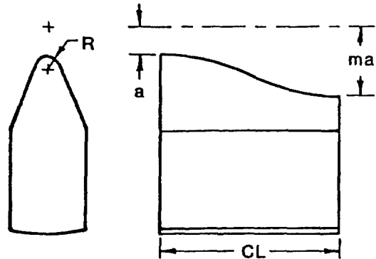
Fig. 3. Vane geometry parameters.
