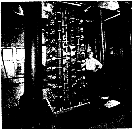
C-W Rear View Showing Spark Gaps
