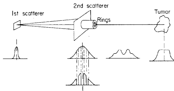
Figure 2. Occluding Ring beam delivery system.
