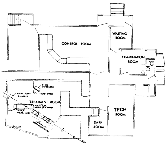
Figure 1. The Bevalac Radiotherapy Facility.
