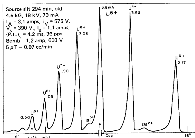
Figure 1. Ion current vs. \rho (radius). Modified GANIL slit, 1.1 x 45 mm; U/Xe; source age: 13 hrs.; cup width: .63 cm.
