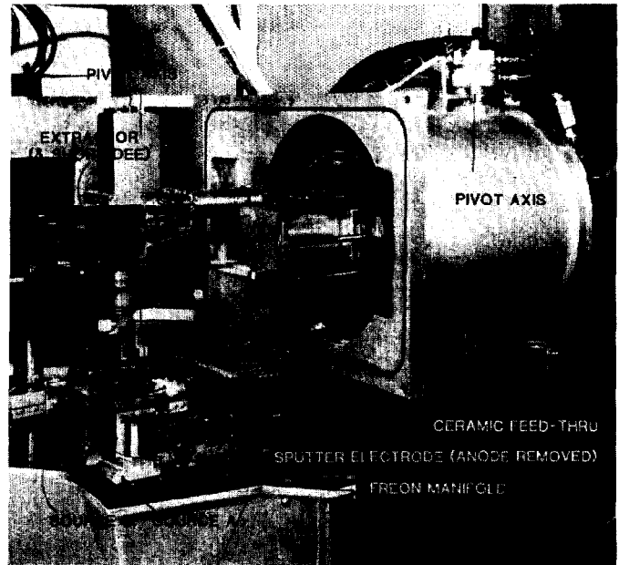
Figure 3. Source swung in open position. Dual head assembly below with one gas cap removed.
