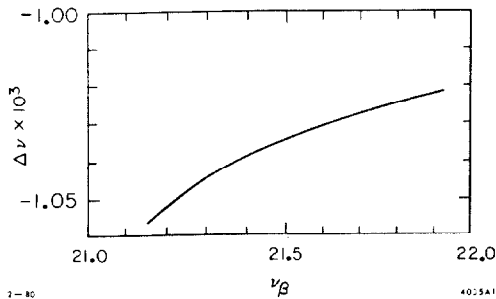
Fig. 1. Coherent betatron tune shift versus the unperturbed betatron tune for the rigid bunch mode m = 0 with a 14.5 GeV, 1 ma single-bunch beam.
