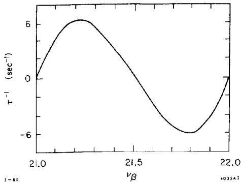
Fig. 2. Instability growth rate (damping rate if negative) versus the unperturbed betatron tune for the rigid bunch mode m = 0 with a 14.5 GeV, 1 ma single-bunch beam. The radiation damping rate at 14.5 GeV is 110 \text{ sec}^{-1} .
