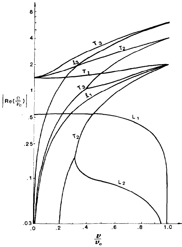
Fig. 1. Real part of the first ten roots of dispersion relation, shown as functions of betatron frequency. Quantities are normalized to the zero current betatron frequency. The transverse modes T_n correspond to Gluckstern's axi-symmetric modes. (1) l_1 and l_3 are the longitudinal modes due to the correlation between the longitudinal velocity and the transverse motion. L_1 is the ordinary longitudinal mode. L_2 is the lowest mode indicated by Eqn. (6).
