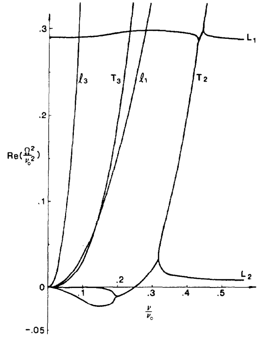
Fig. 2. Real part of the square of the Doppler shifted frequency ( \Omega = \omega - kv_0 ) versus betatron frequency in the high density-low frequency domain. Quantities are normalized to \nu_0^2 and \nu_0 respectively.
