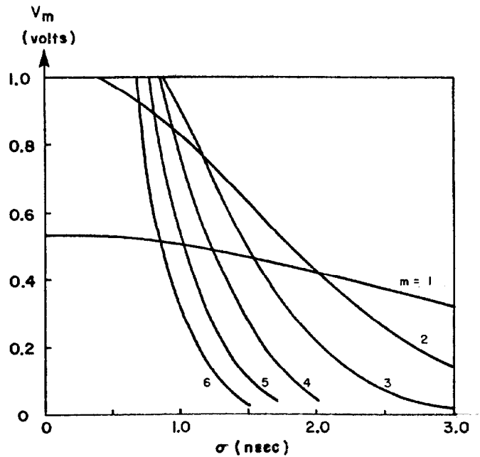
FIGURE 2. Peak voltage output for pickup electrode signal into 50 ohms, vs RMS proton bunch width, for various harmonics of 53 MHz, at 10^{10} protons/bunch.
