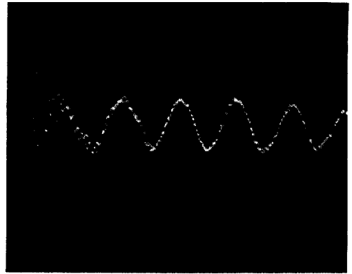
FIGURE 4. Horizontal beam position vs time for beam injected into Main Ring. Vertical axis is 500 microns per major division. Horizontal axis is 1 msec per major division. The synchrotron oscillation frequency is about 600 Hz. The RMS resolution is about 30 microns.
