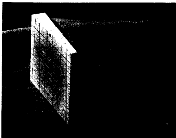
Figure 1. Aluminum range-measuring wedge. The fiducial pattern machined on the back face of the wedge will be imprinted by the beam on photographic film placed against it.
