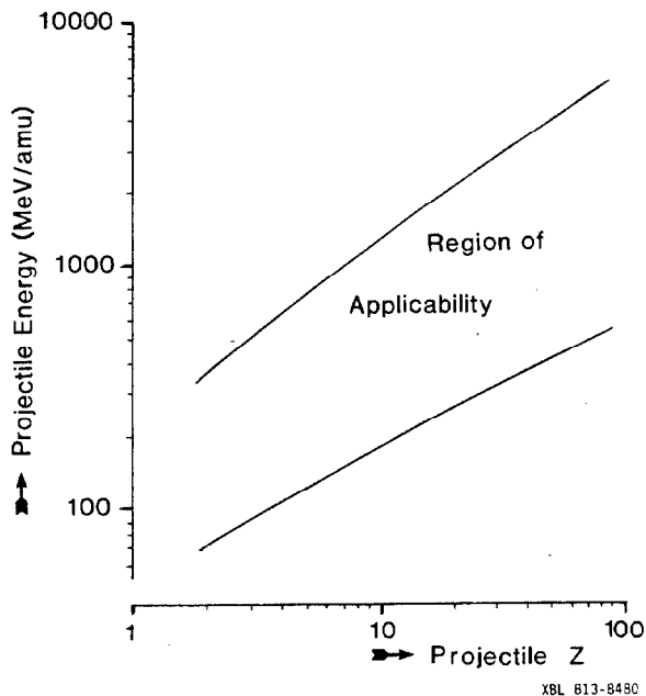
Figure 3. Region where the range-measurements discussed here provide good information about beam energy. At the low end a sufficient amount of material must be penetrated to expose the film, while multiple scattering, straggling and nuclear attenuation limit the upper end.
