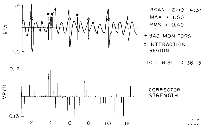
Fig. 3. Typical vertical dispersion function before correction.
