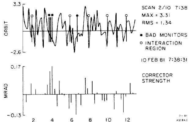
Fig. 1. Typical vertical orbit for an operating PEP configuration.
