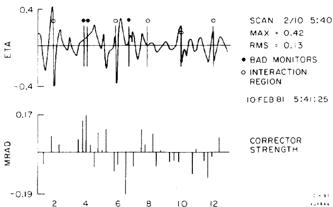
Fig. 4. Vertical dispersion function after correction.
