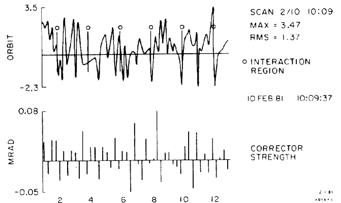
Fig. 2. Vertical orbit after global correction using method 2.
