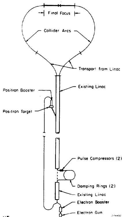
Fig. 1. Layout of the SLAC Linear Collider.
