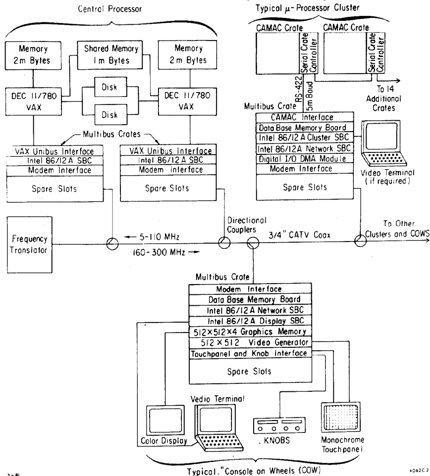
Fig. 2. SLC Computer System Block Diagram.
