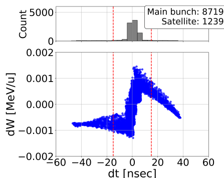
Figure 9: Longitudinal phase space of the bunch before the Quadrupole triplet entrance with the kicker.
