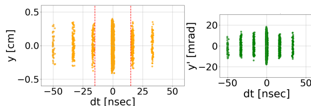
Figure 11: Transverse longitudinal correlation downstream of the RFQ without the kicker.
