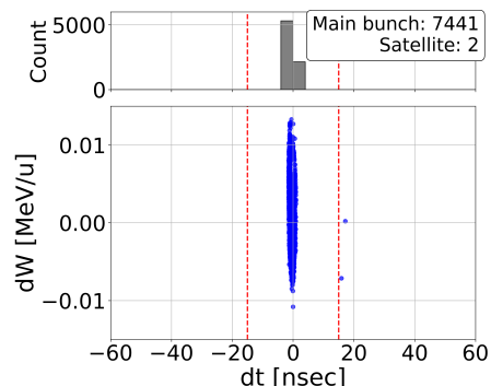
Figure 10: Longitudinal phase space of the bunch downstream of the RFQ with the kicker.
