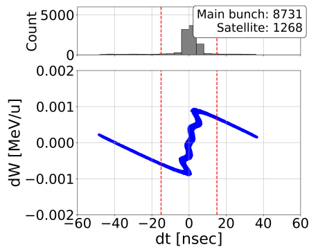
Figure 3: Longitudinal Phase space at the entrance of the Quadrupole triplet.
