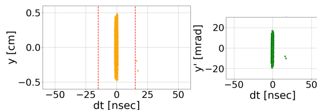
Figure 12: Transverse-longitudinal correlation downstream of the RFQ with the kicker.
