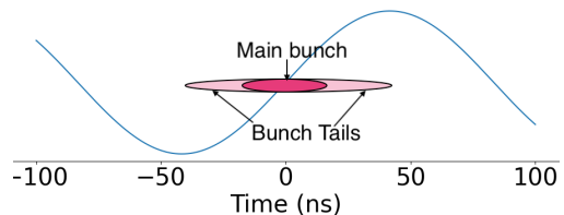
Figure 5: Bunch cleaning with a 6 Mhz E-field.
