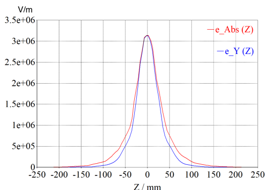
Figure 7: E-field profile on the beam axis.
