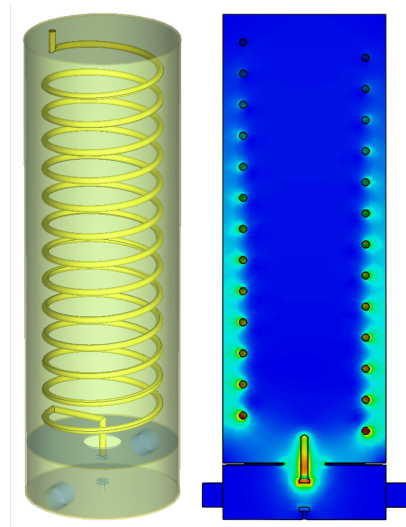
Figure 6: CST model of the RF-kicker. (left) Modeled kicker geometry. (right) Electric field distribution on the cut section.
