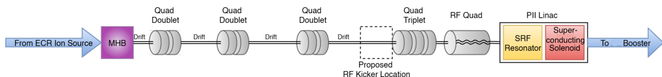
Figure 1: The Low Energy Beam Transport (LEBT) section of the ATLAS facility.
