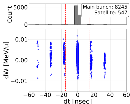
Figure 4: Longitudinal phase space of the bunch after RFQ.
