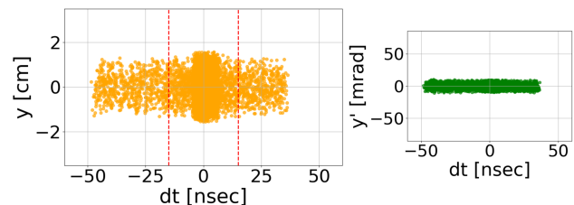
Figure 2: Transverse longitudinal correlations plotted at the entrance of quadrupole triplet magnet.
