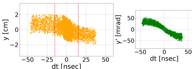
Figure 8: Transverse longitudinal correlation after the kicker.
