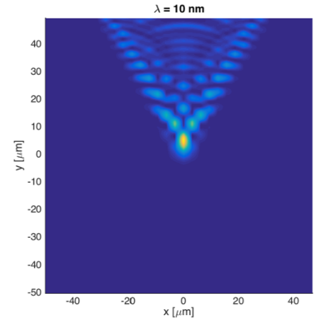
Toroidal aberration
