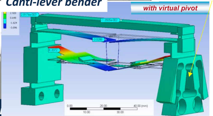
Canti-lever bender
