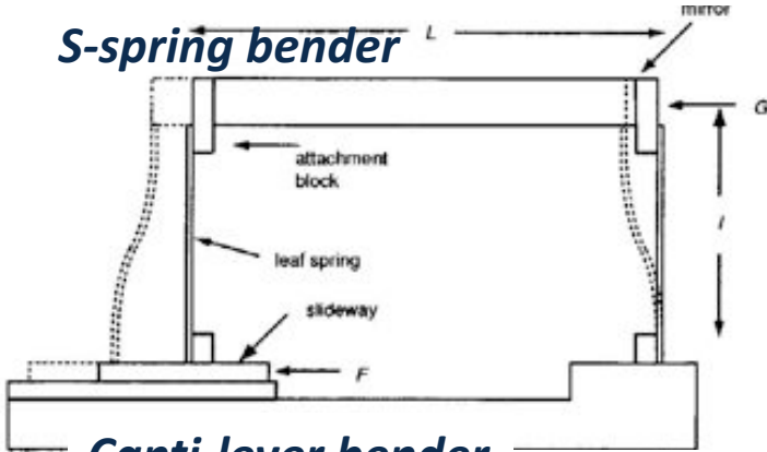
Canti-lever bender
