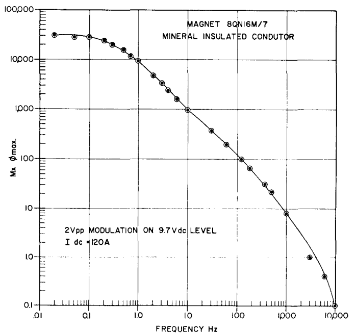
Fig. 7 Ripple flux vs frequency for 2 Vpp voltage modulation on magnet 8Q16M/7
