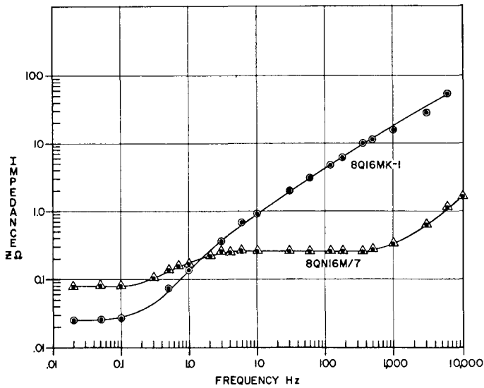
Fig. 4 Impedance vs frequency
