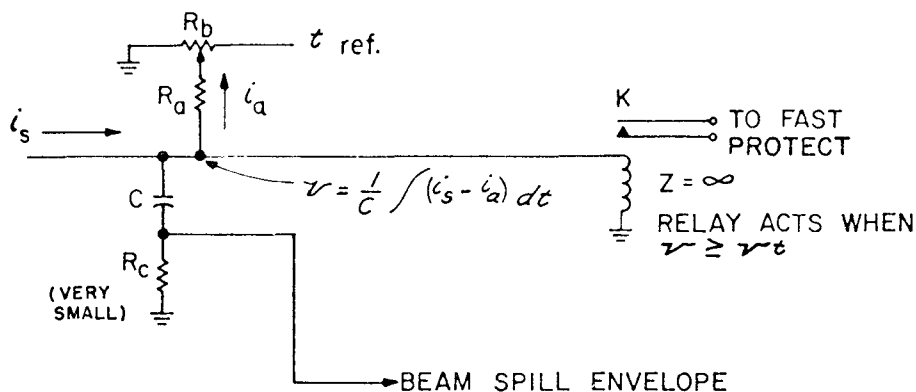
Fig. 1 Conceptual beam spill control system
