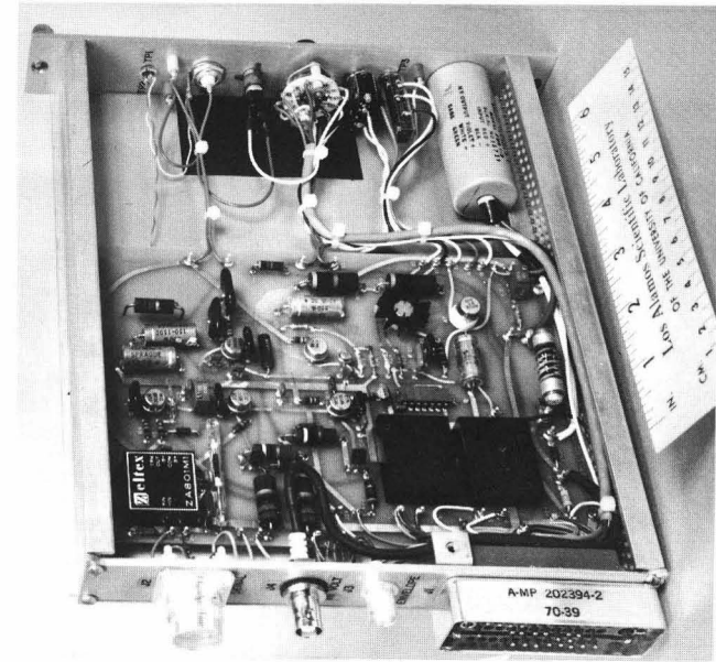
Fig. 4 Control system NIM module
