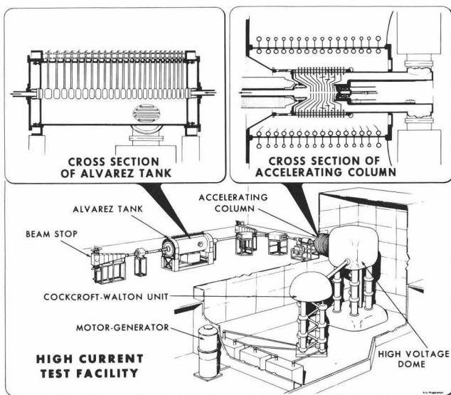
Fig. 1. General view of high current test facility.
