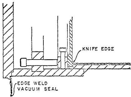
Fig. 16. Rf edge seal between end plate and tank wall.
