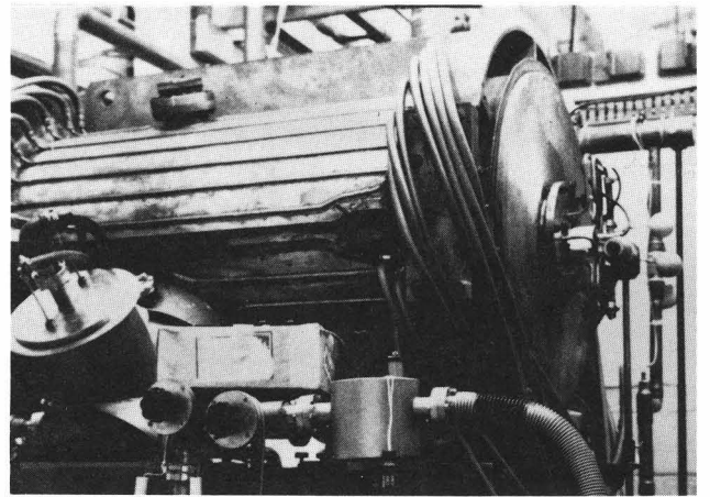
Fig. 13. 100% duty factor short tank.
