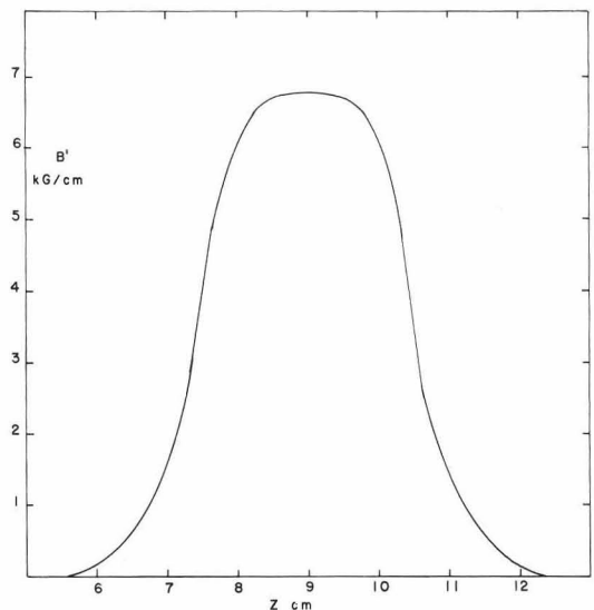
Fig. 9. Axial field gradient for drift tube quadrupole magnet.
