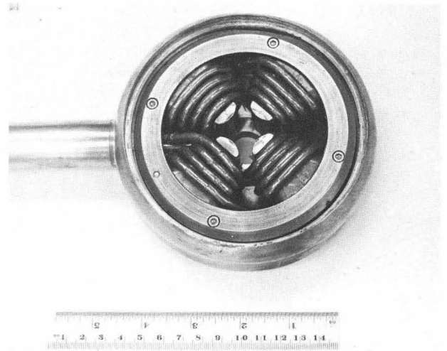
Fig. 8. Drift tube with magnet.
