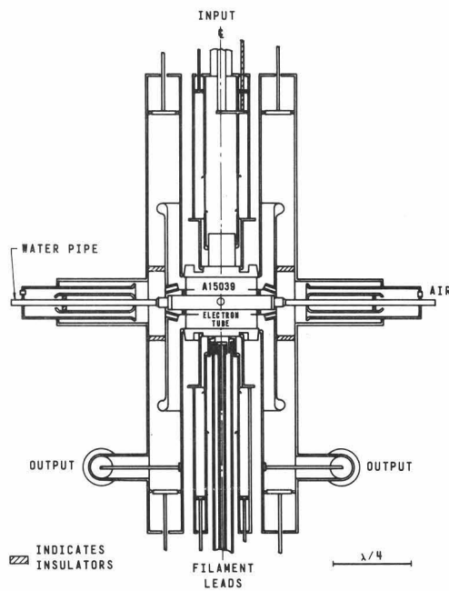
Fig. 11. A15039 amplifier structure.
