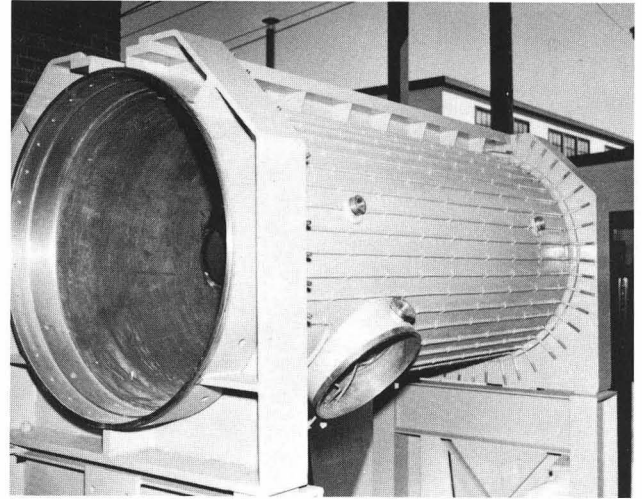
Fig. 7. Alvarez tank.
