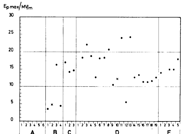
Fig. 5. Peak electric fields at breakdown for resonators B to E.
