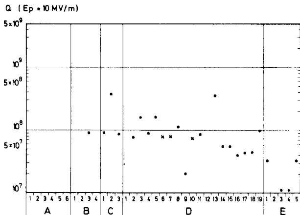
Fig. 4. Q at high field strength ( E_p = 10 \text{ MV/m} ) for resonators B to E.
