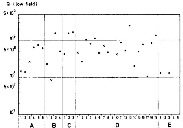
Fig. 3. Low field Q in different test runs.
