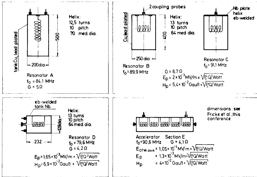
Fig. 1. Resonators A to E and their essential parameters.
