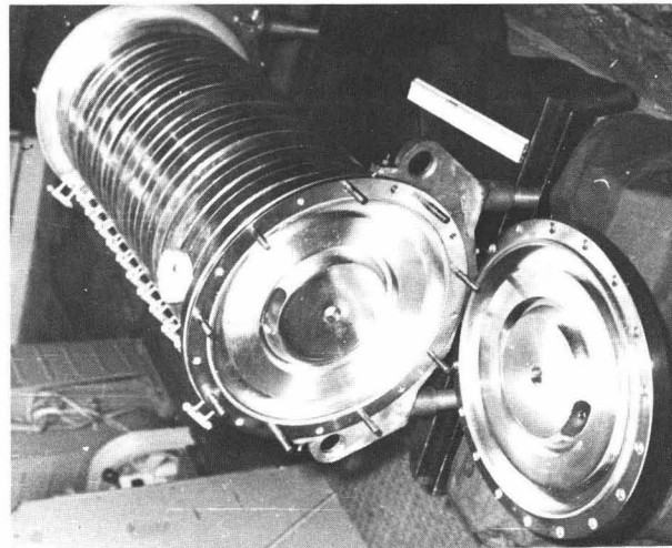
Fig. 4 Model of accelerating structure with annular coupling cavities.
