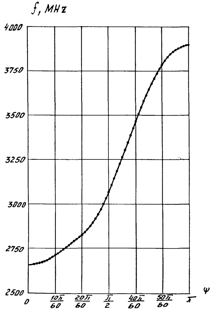
Fig. 9 Dispersion curve of disc-and-washer loaded structure
