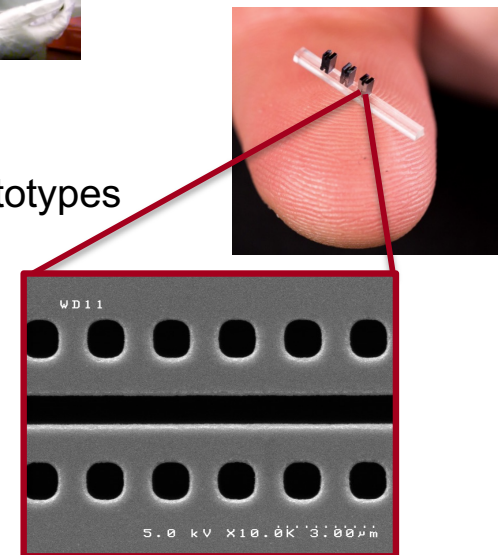
silicon
