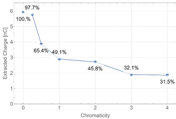
Figure 5: Extracted charge and transfer efficiency as a function of chromaticity. In all cases, the bunch distribution for an 8 A (16 pC) bunch out of the gun was used.
