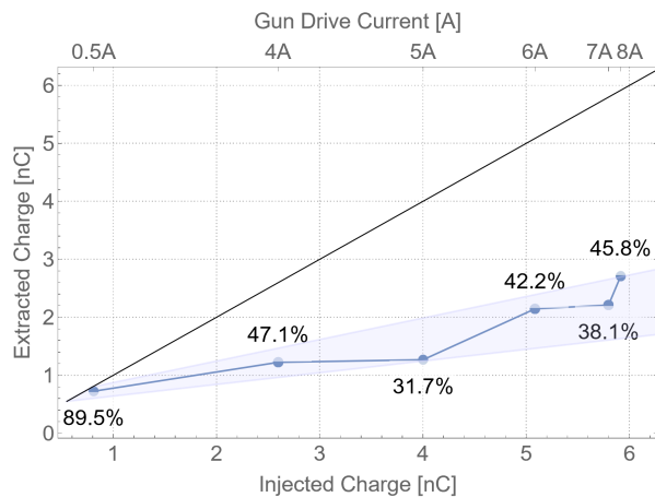
Figure 4: Extracted charge and transfer efficiency as a function of charge at injection into the booster (central S-band bunch only). The black line indicates 100 % transfer efficiency.
