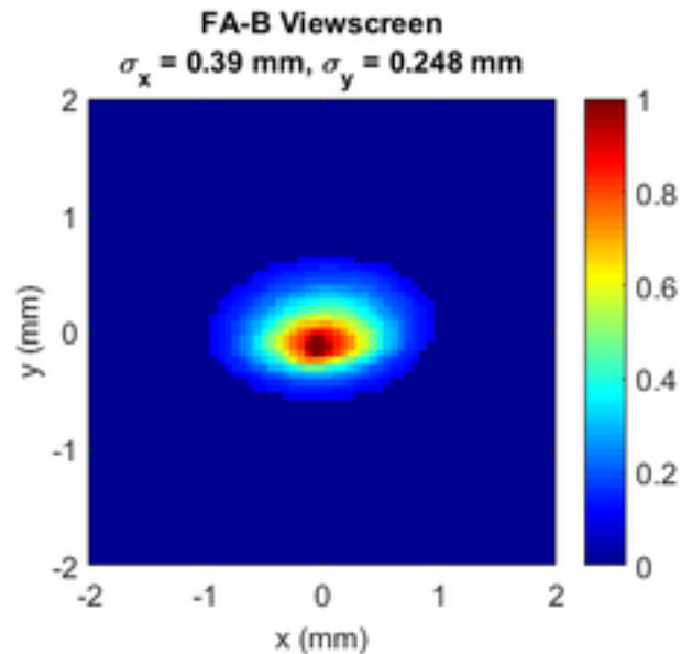
Figure 6: First 42-MeV beam spot observed at the end of the F.A.T. line.
