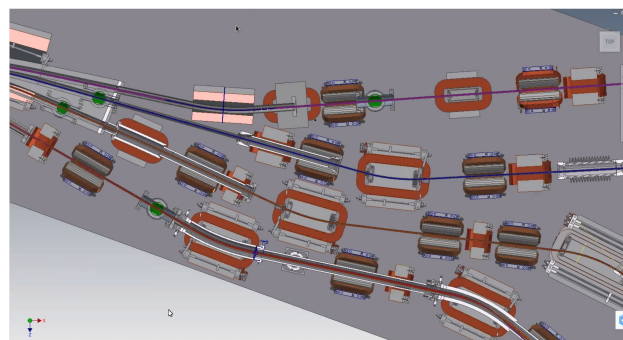
Figure 1: Schematic diagram of the upstream half of the splitter section SX downstream of the main linac. Dipole magnets are shown in gray/orange; the quadrupoles are shown in gray/blue. The areas in pink will be occupied by septum magnets.
