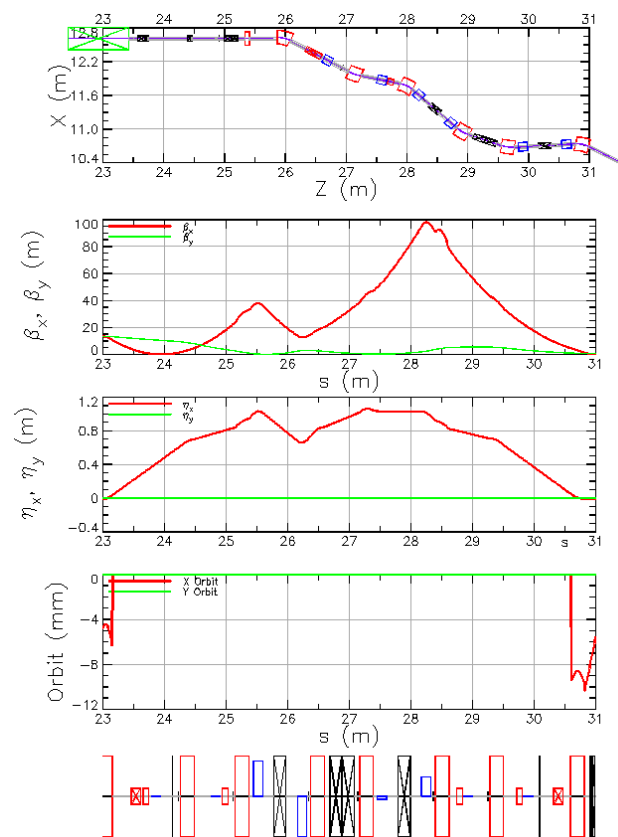
Figure 5: Twiss functions for the four-quadrupole S1 line optics.
