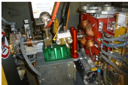
Figure 5: BLMs in undulator section (S1).
