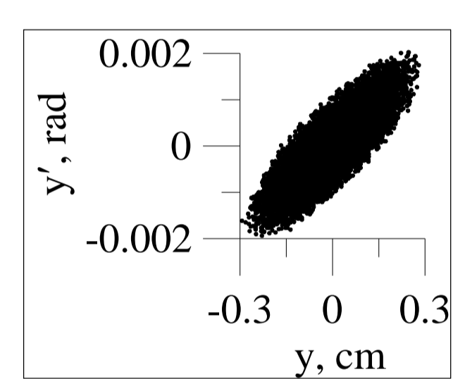
Figure 16: Plane ( y, y' )
