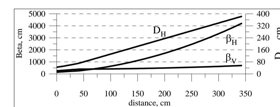
Figure 18: The betatron \beta_{H,V} and dispersion D_H functions along the experimental beamline at 24 MeV.
