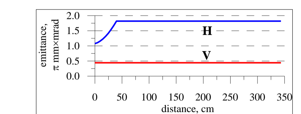
Figure 19: The horizontal (H) and vertical (V) rms beam emittance along the experimental beamline.
