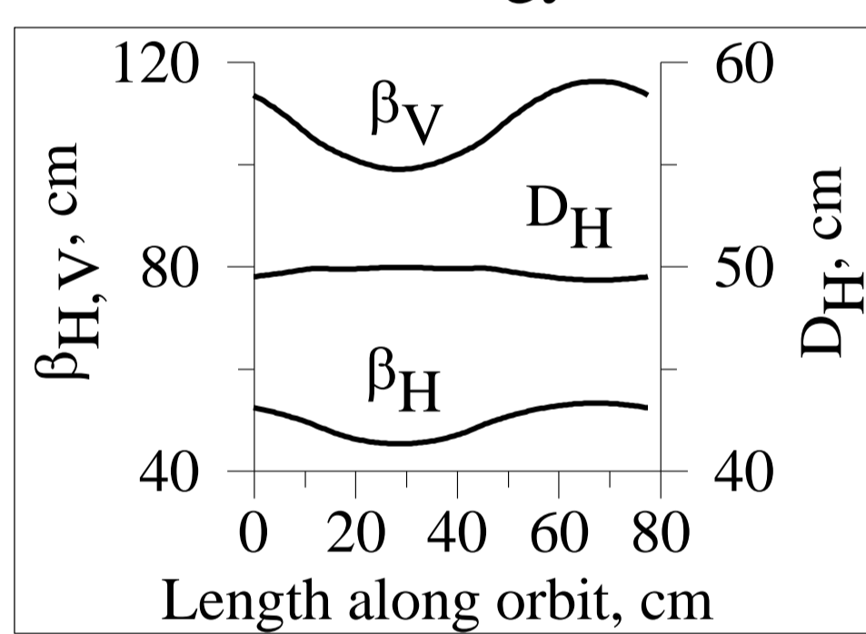
Figure 6: Periodic solutions for \beta_{H,V} and D_H . W_{ex} = 24 MeV.
