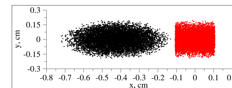
Figure 8: Plane ( x, y ). Accelerated beam - left, stripping foil - right.
