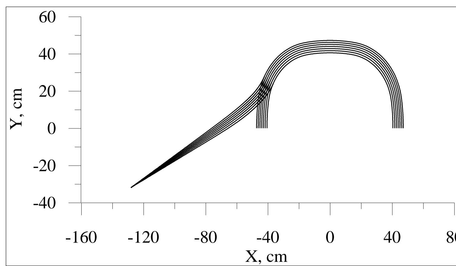
Figure 3: Closed and extraction orbits for extraction energy range 18 MeV \leq W_{ex} \leq 24 MeV.
