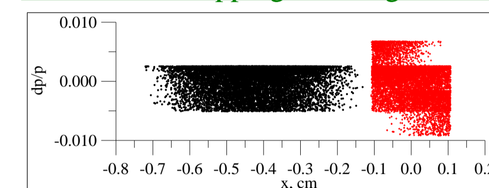
Figure 10: Plane ( x, dp/p ). Accelerated beam - black dots, foil - red dots.
