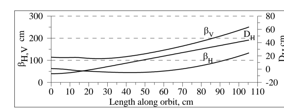
Figure 12: The betatron \beta_{H,V} and dispersion D_H functions along the extraction orbit
