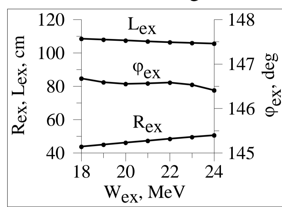
Figure 7: Extraction radius R_{ex} , angle \phi_{ex} and orbit length L_{ex} .
