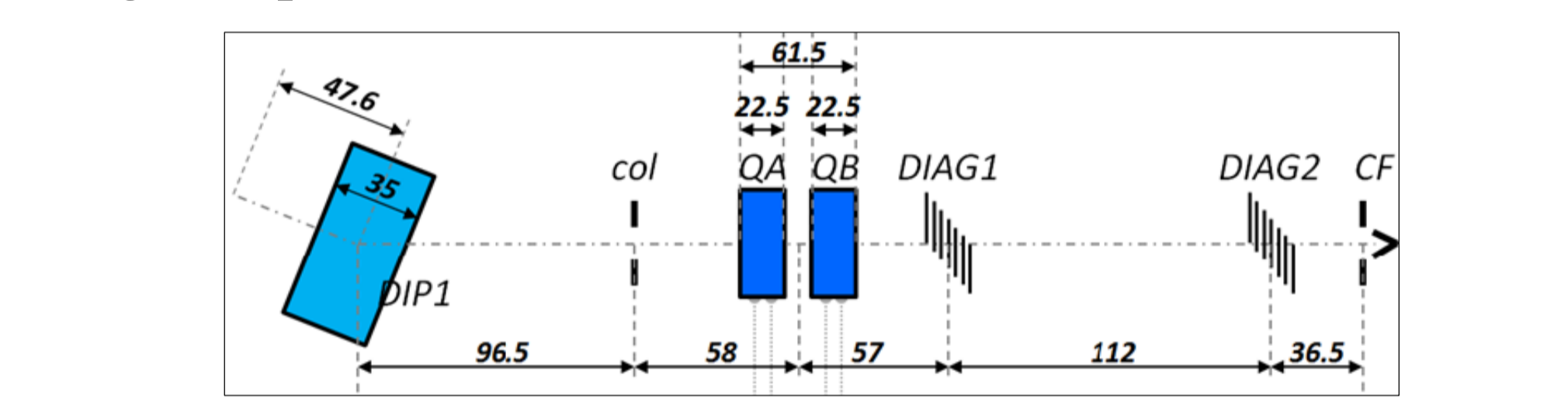
Figure 17: Experimental beam line [4]. DIP1 - combo magnet; QA, QB - quadrupole lenses; DIAG1, 2 - diaphragms, CF - Faraday's cap
