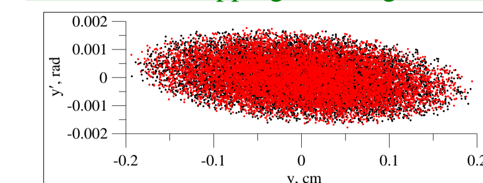
Figure 11: Plane ( y, y' ). Accelerated beam - black dots, foil - red dots.
