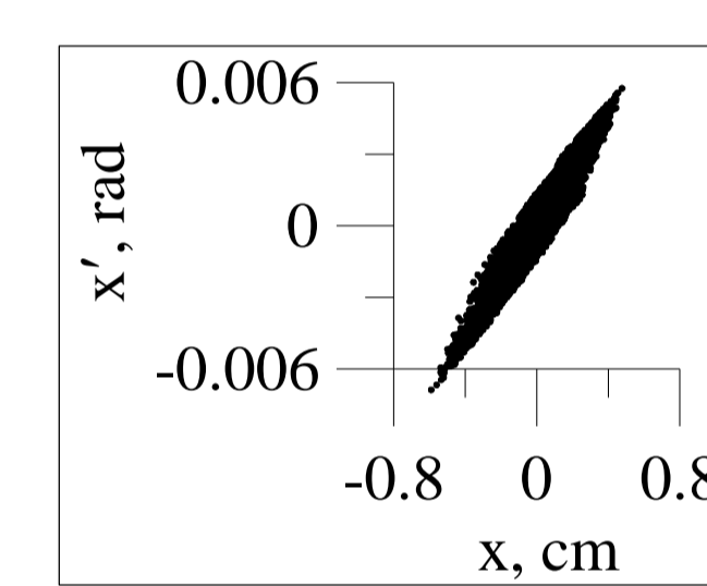
Figure 15: Plane ( x, x' )
