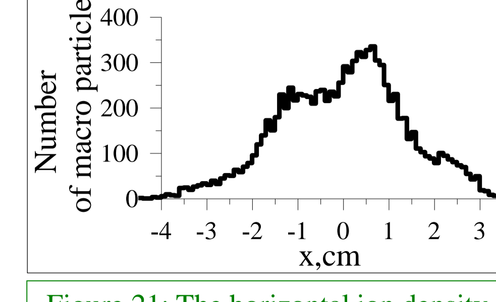
Figure 21: The horizontal ion density at DIAG2
