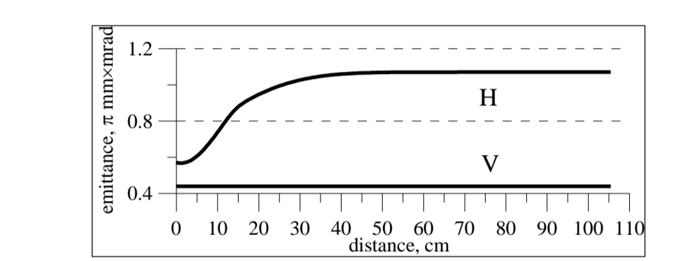
Figure 13: The horizontal (H) and vertical (V) rms beam emittance along the extraction orbit
