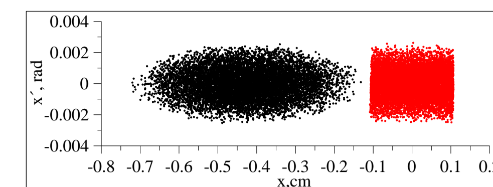
Figure 9: Plane ( x, x' ). Accelerated beam - left, stripping foil - right.
