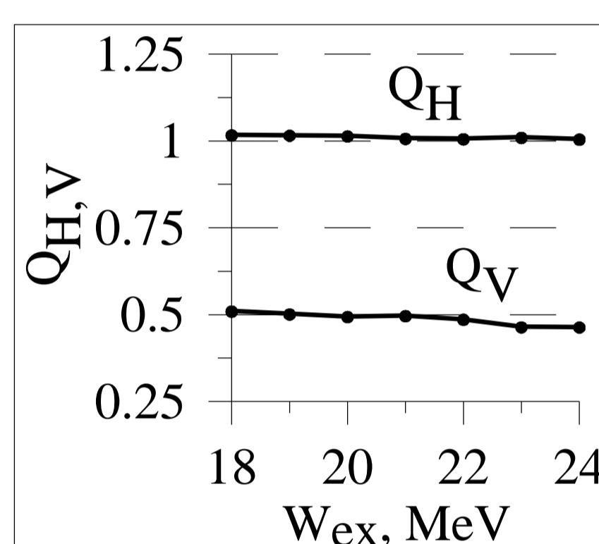
Figure 4: Frequencies Q_{H,V} .
