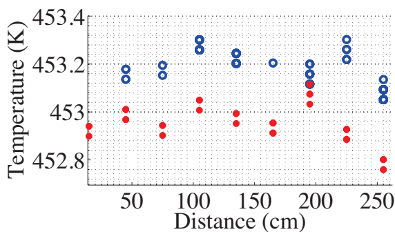
Figure 3: Temperature profiles measured along the heat exchanger. The blue circles correspond to the normal configuration where the oil is pumped in from the sides and goes out in the middle. The red stars correspond to the modified heater where the oils is pumped in from one end and goes out at the other end. In both cases the measurements remain within \pm \sim 0.1 K.
