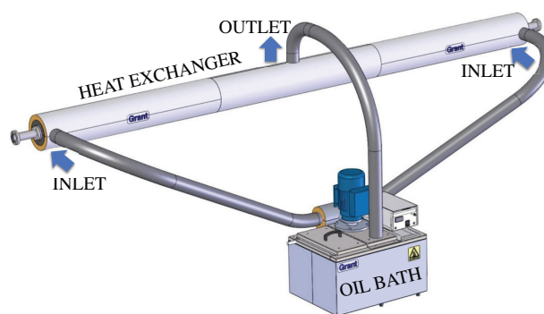
Figure 2: A CAD drawing of the oil heating system which consist of an oil bath and a heat exchanger (Courtesy of Grant Instruments, UK).
