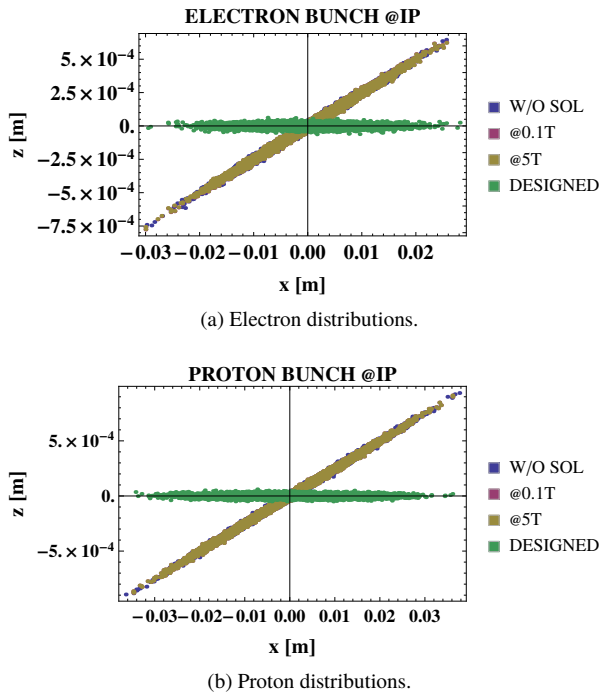
Figure 5: Electron (a) and proton (b) distributions at the IP for different B_{Sol} , using a crabber rotated by an angle of KL , compared to the case of the solenoid off (blue), and both the crabbing cavity and the solenoid off (green).
